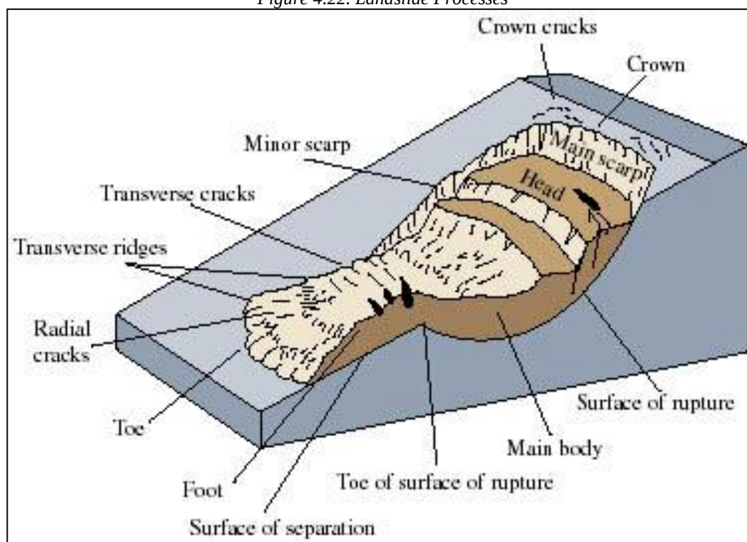
Figure 4.22. Landslide Processes
